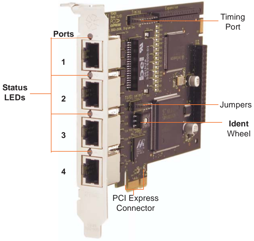
Figure 5: TE420 Card
